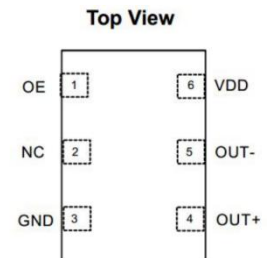
Figure 1. Pin Assignments
