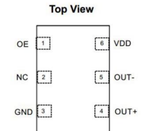
Figure 1. Pin Assignments
