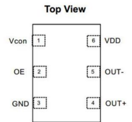
Figure 1. Pin Assignments
