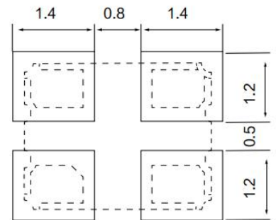
TOP View Suggested Layout
