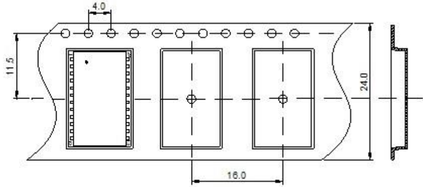
Tape & Reel
