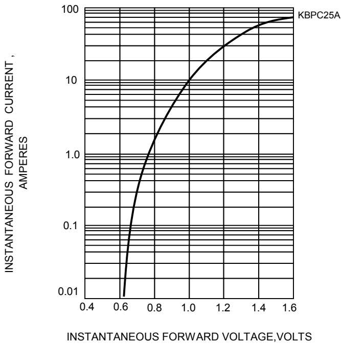
FIG.3-TYPICAL FORWARD CHARACTERISTICS
