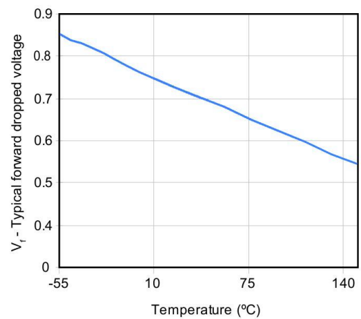
Figure 6 - Forward Voltage
