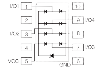
DFN-10-2.5×2.5×0.6-0.5(Top view)
