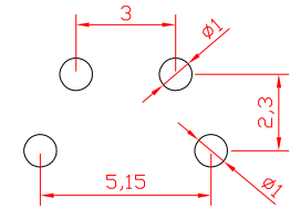
PCB. WELDING DRAWING
