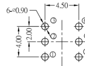
P.C.B.LAYOUT(TOP VIEW)
