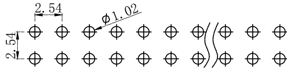
PCB LAYOUT
