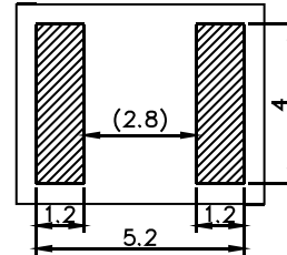
Recommended pad outline
