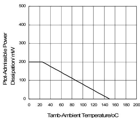
Figure 2. Power De-rating
