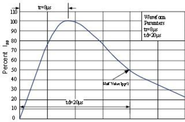
Figure 5: Pulse Waveform
