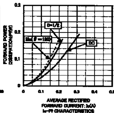
I-F CHARACTERISTICS
