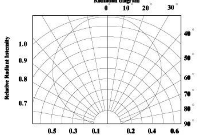
Radiation diagram
