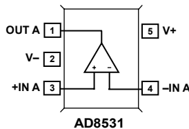
Figure 1. 5-Lead SC70 and 5-Lead SOT-23 (KS and RT Suffixes)
