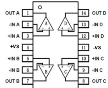
8544A TSSOP-14/SOP-14
