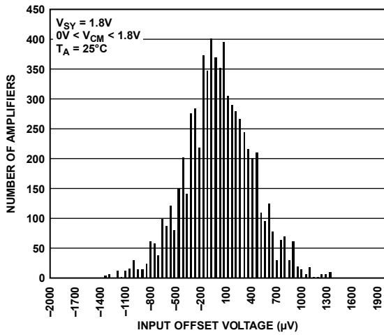
Figure 27. Input Offset Voltage Distribution
