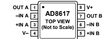
Figure 2. 8-Lead MSOP and 8-Lead SOIC_N
