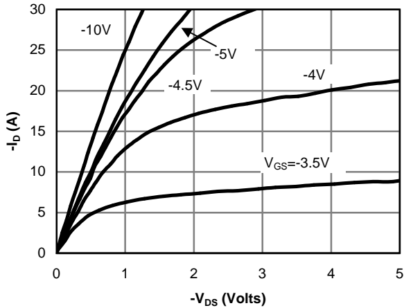
Fig 12: On-Region Characteristics
