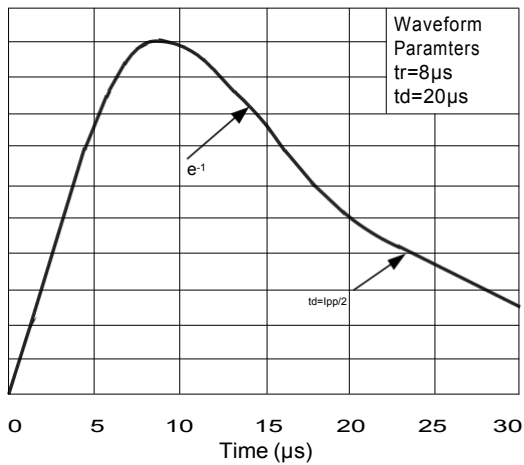
Figure3: Pulse Waveform
