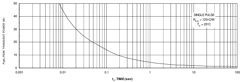
Figure 11. Single Pulse Maximum Power Dissipation.
