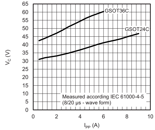
Fig. 9 - Typical Peak Clamping Voltage vs. Peak Pulse Current
