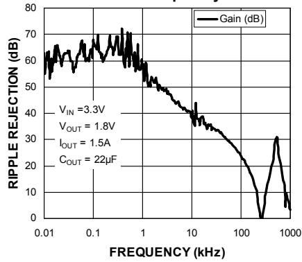
Ripple Rejection ( I_{OUT} = 1.5A ) vs. Frequency
