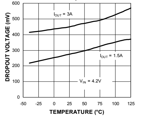
Dropout Voltage vs. Temperature
