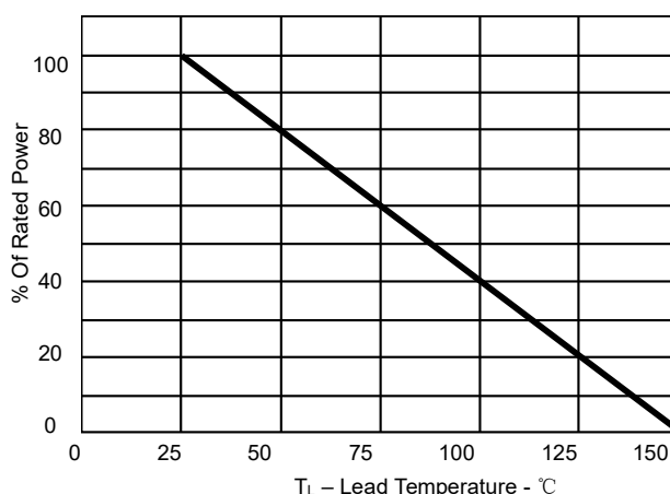
Fig 2.Power Derating Curve
