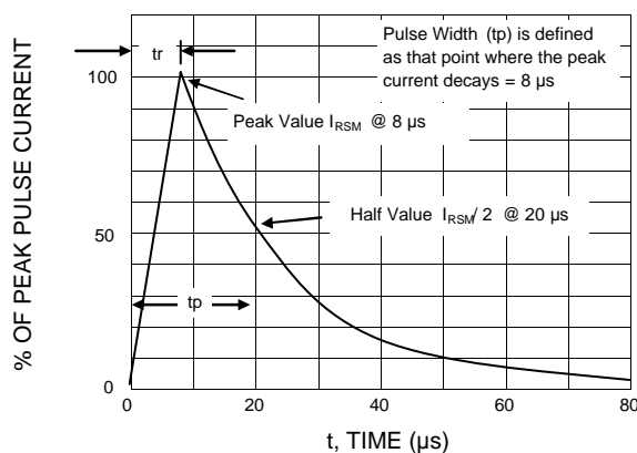
FIG.5 - 8 x 20 \mu s PULSE WAVEFORM
