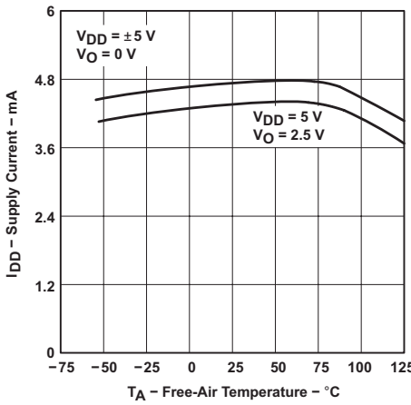
Figure 39. TLC2274 Supply Current vs Free-Air Temperature
