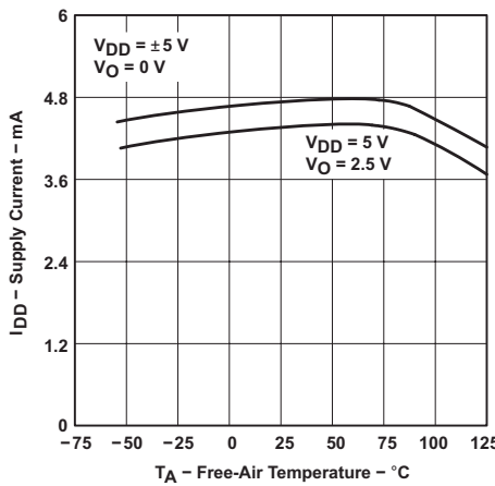
Figure 39. TLC2274 Supply Current vs Free-Air Temperature
