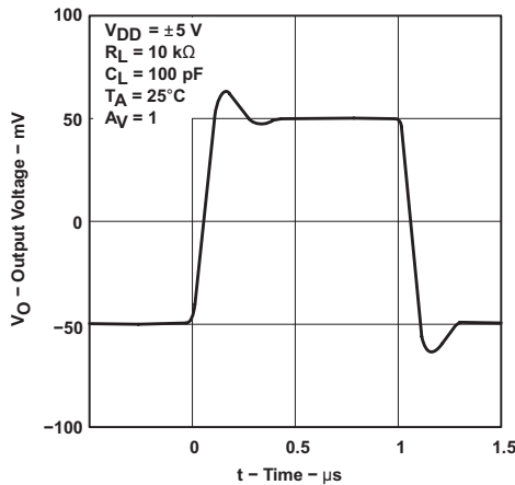
Figure 49. Voltage-Follower Small-Signal Pulse Response
