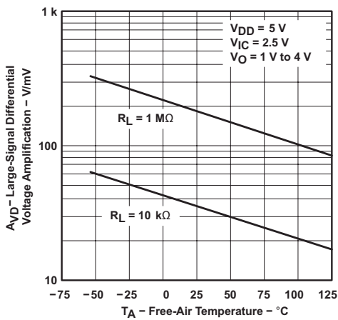
Figure 27. Large-Signal Differential Voltage Amplification vs Free-Air Temperature
