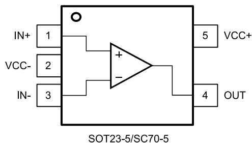
Package pin connections (top view)
