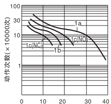
触点电流(A)
