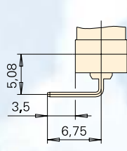
PCB terminal 0,6 x 0,5 mm LH-side w/o location pins
