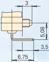
PCB terminal 0,6 x 0,5 mm RH-side with location pins
