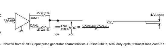
F8. Common Mode Output Voltage Test and Voltage Waveform
