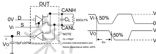
F7. tEN Test Circuit and Voltage Waveforms
