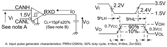
A. Input pulse generator characteristics: PRRs125KHz, 50% duty cycle, tr<6ns, tf<6ns, Zo=50Ω; B. CL includes instrumentation and fixed capacitance within 20% error;
