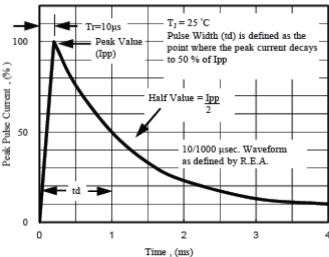
Fig. 5 - Pulse Waveform
