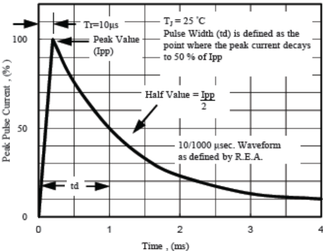
Fig. 5 - Pulse Waveform
