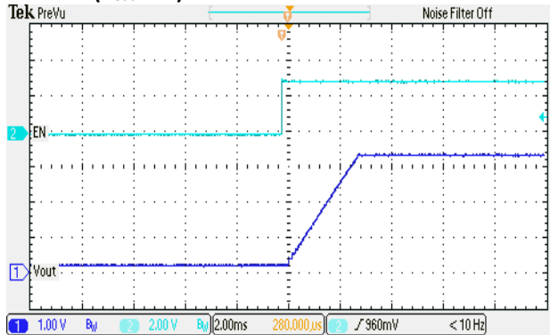
Start UP ( I_{Load}=1A )
