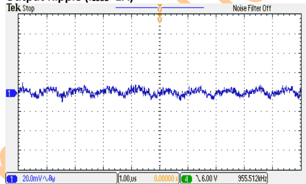
Output Ripple ( I_{Load}=1A )
