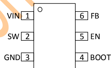
Top View SOT563 (1.6mm x 1.6mm)
