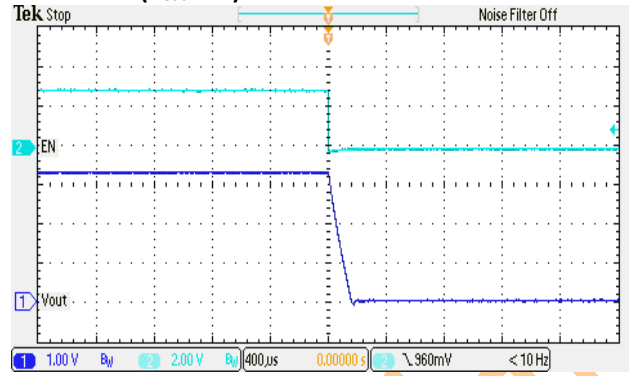
Shut Down ( I_{Load}=1A )
