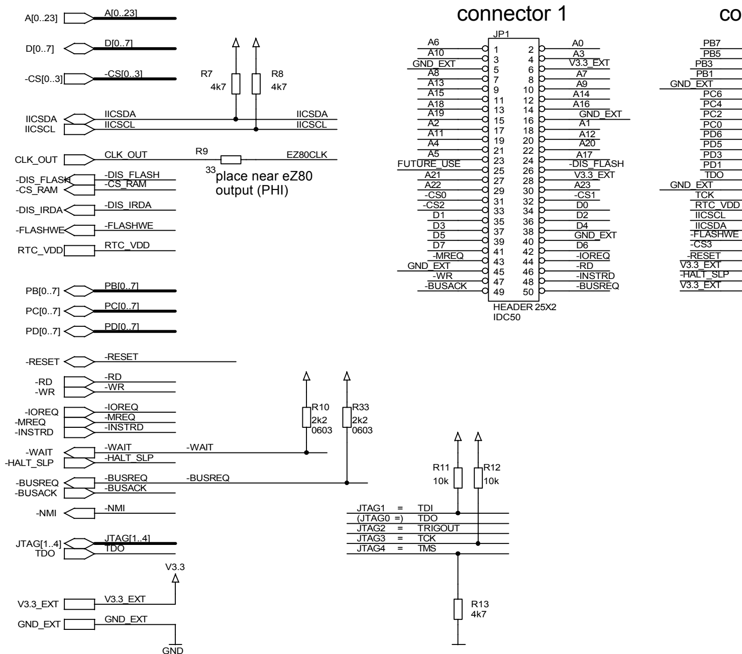
Figure 28. Schematic Diagram, #7 of 9—Headers
