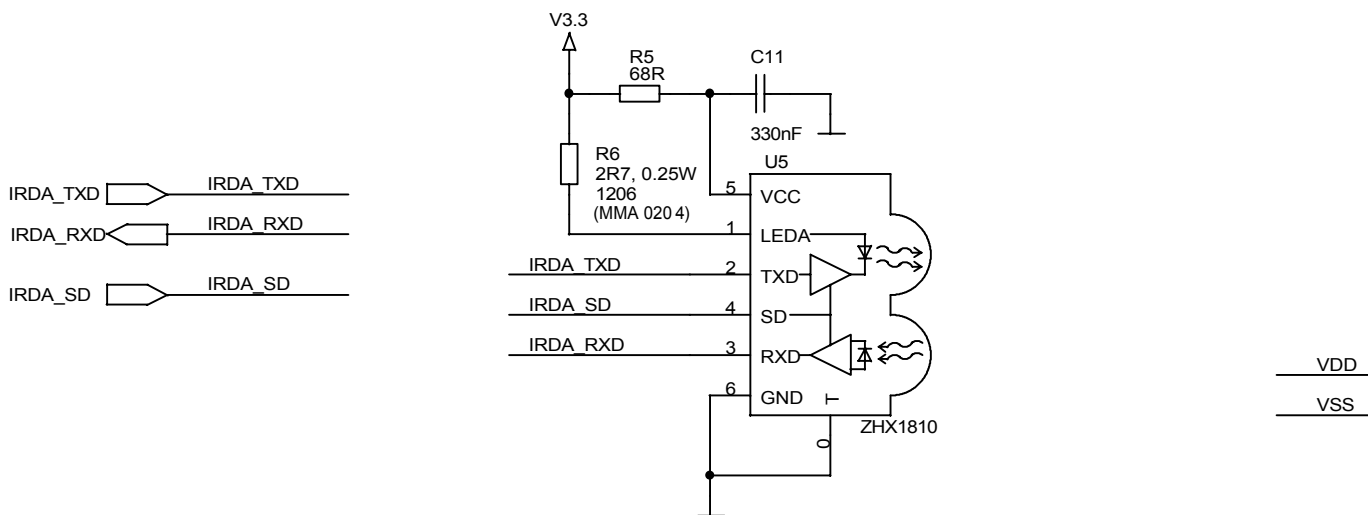
Figure 27. Schematic Diagram, #6 of 9—IrDA Reset
