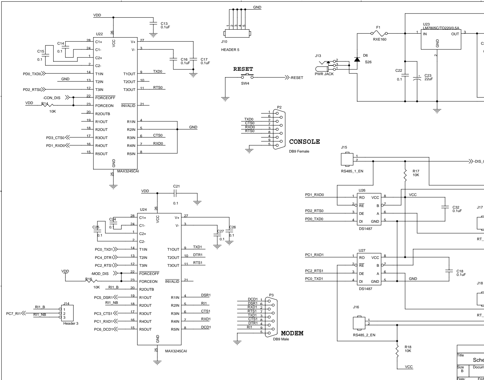
Figure 20. eZ80Acclaim!® Development Platform Schematic Diagram, #4 of 4
