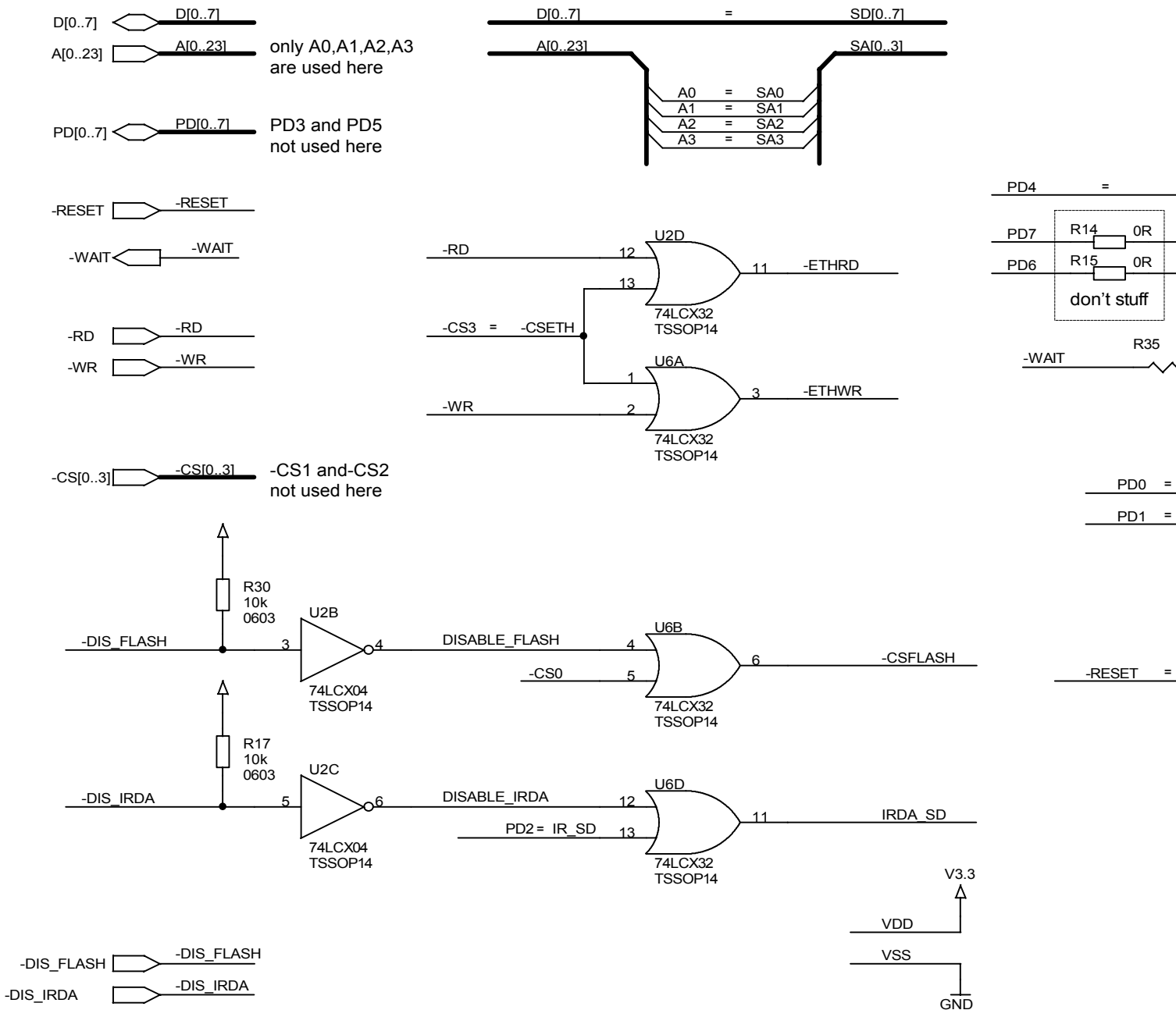
Figure 30. Schematic Diagram, #9 of 9—Control Logic
