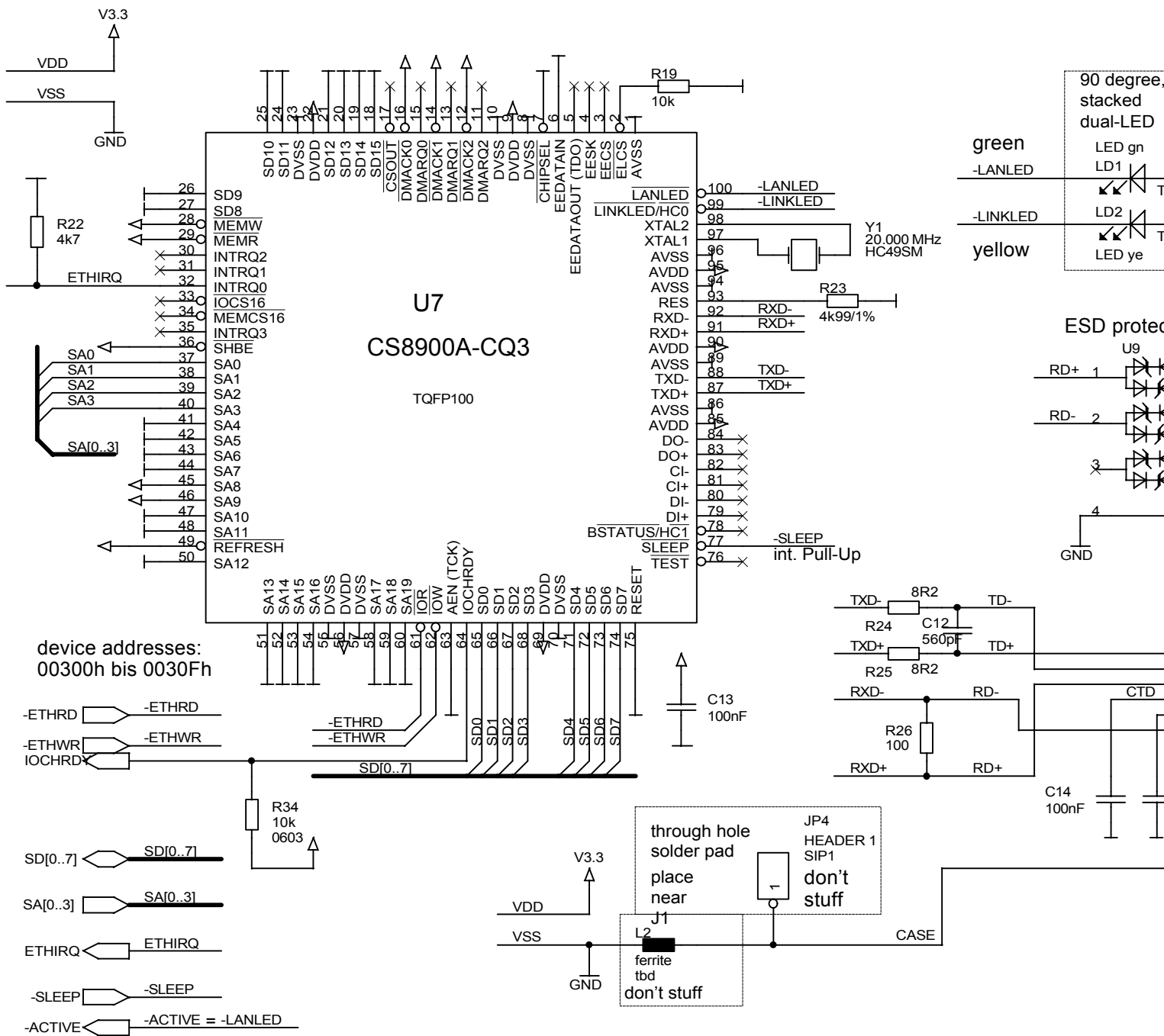
Figure 26. Schematic Diagram, #5 of 9—eZ80F92 Flash Module
