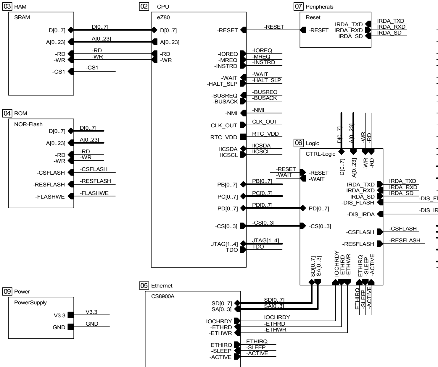
Figure 22. Schematic Diagram, #1 of 9—Top Level
