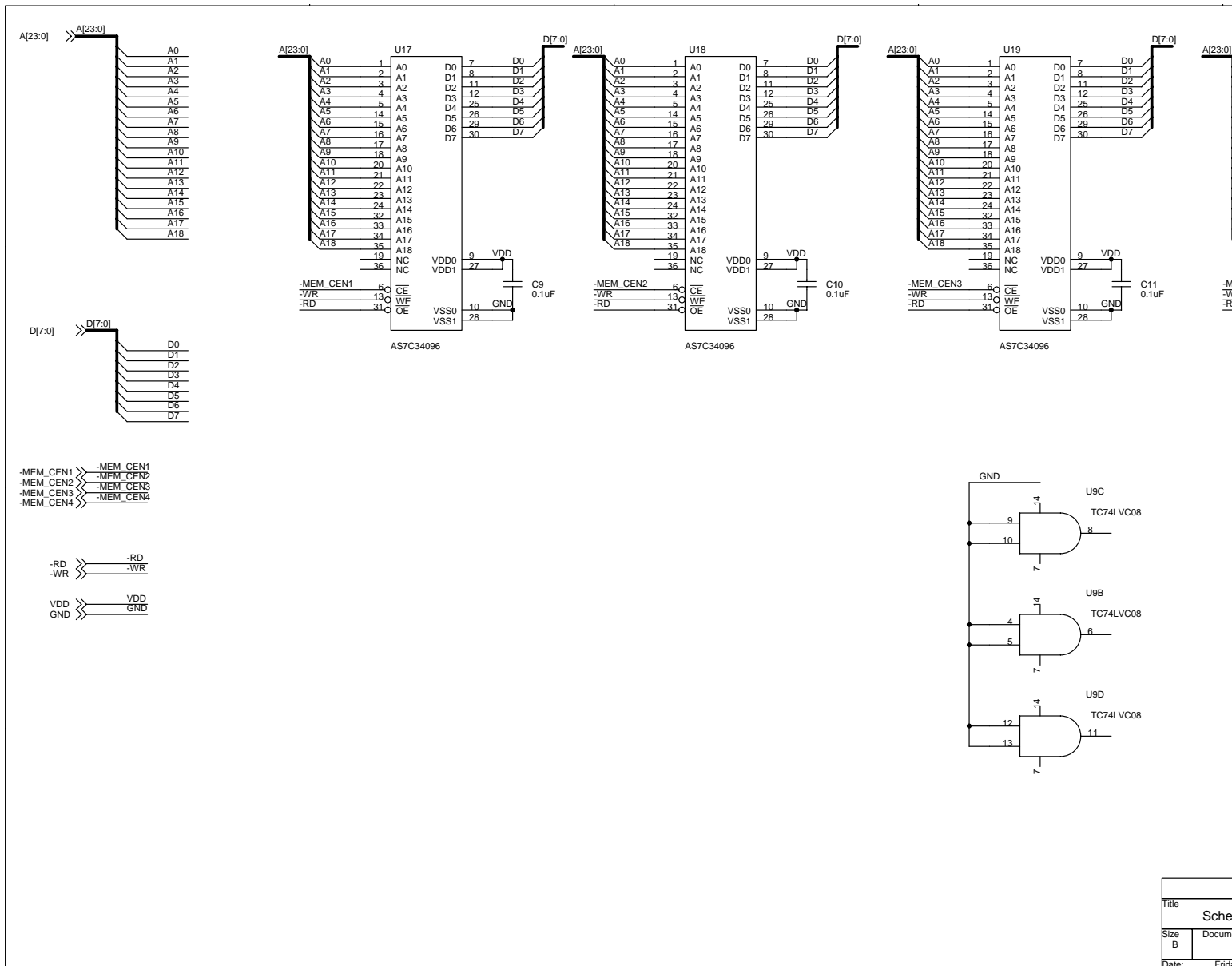
Figure 19. eZ80Acclaim!® Development Platform Schematic Diagram, #3 of 4
