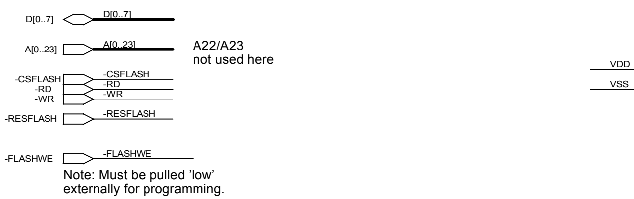
Figure 25. Schematic Diagram, #4 of 9—NOR Flash Device
