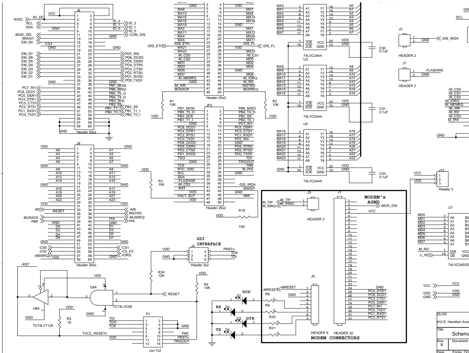
Figure 17. eZ80Acclaim!® Development Platform Schematic Diagram, #1 of 4
