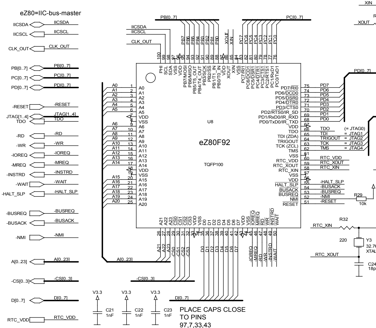
Figure 23. Schematic Diagram, #2 of 9—100-Pin QFP eZ80F92 Device
