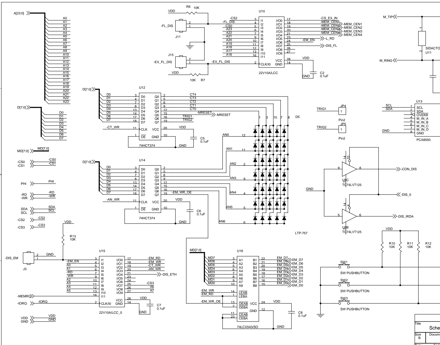
Figure 18. eZ80Acclaim!® Development Platform Schematic Diagram, #2 of 4
