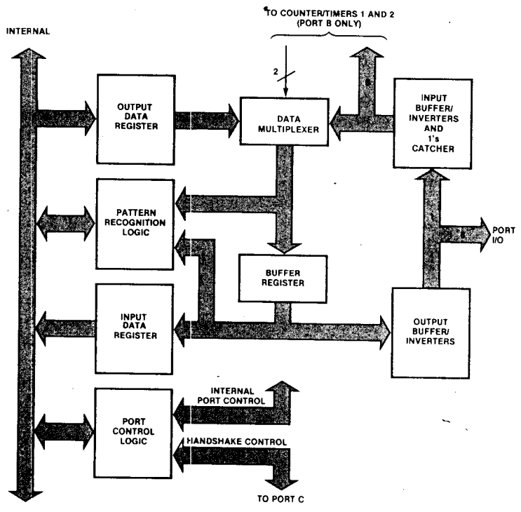
Figure 1-2. Ports A and B Block Diagram
