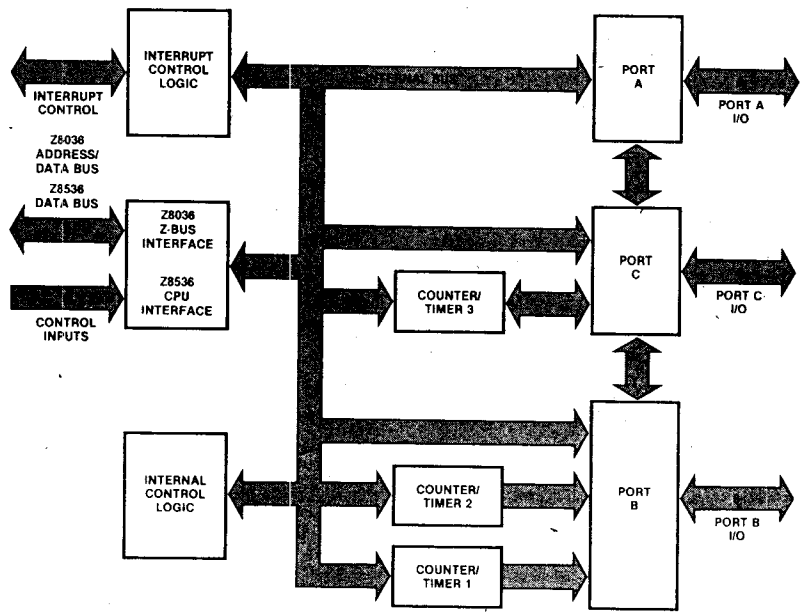
Figure 1-1. Z8036/Z8536 Z-CIO/CIO Block Diagram
