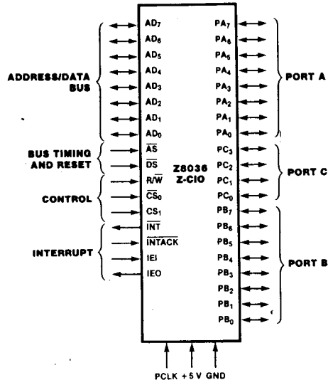
Figure 1. Pin Functions
