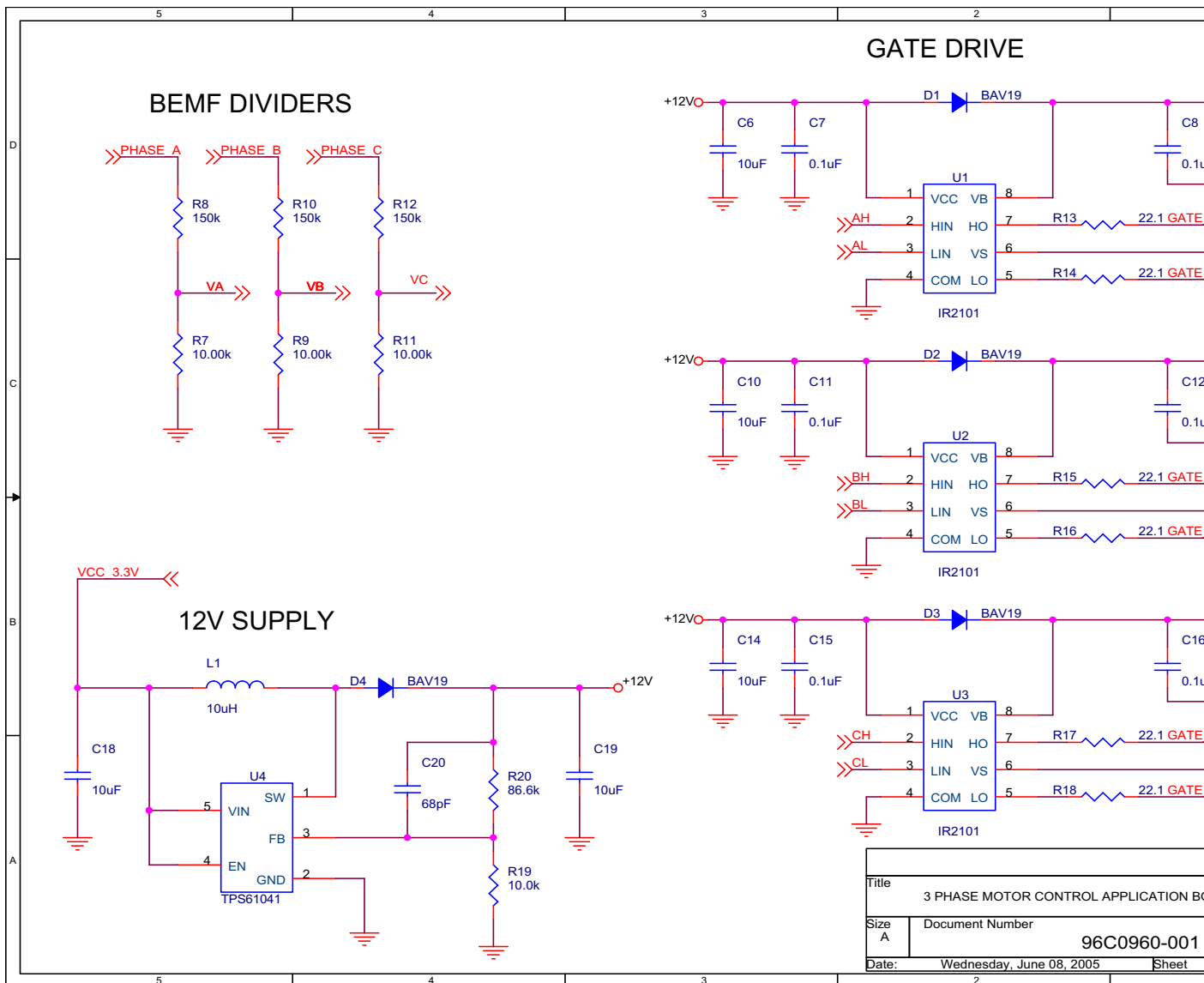
Figure 8. 3-Phase Motor Control Application Board Schematic, #2 of 3
