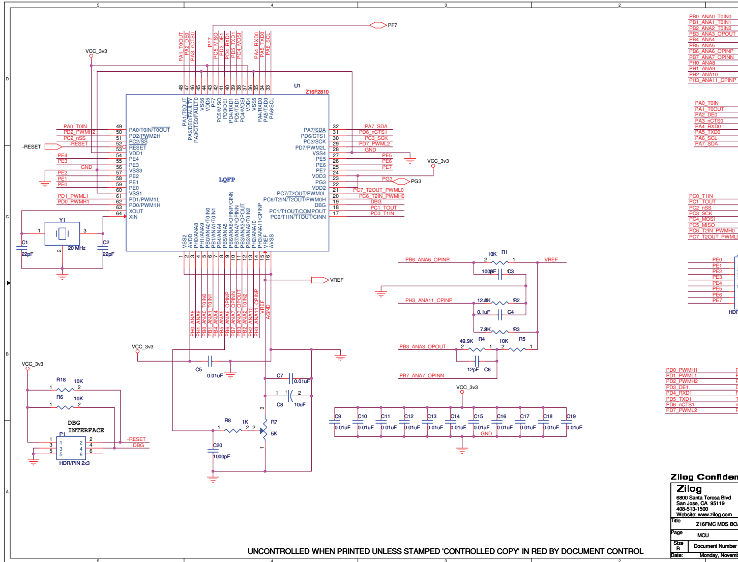
Figure 10. Z16FMC MDS Board Schematic, #1 of 3
