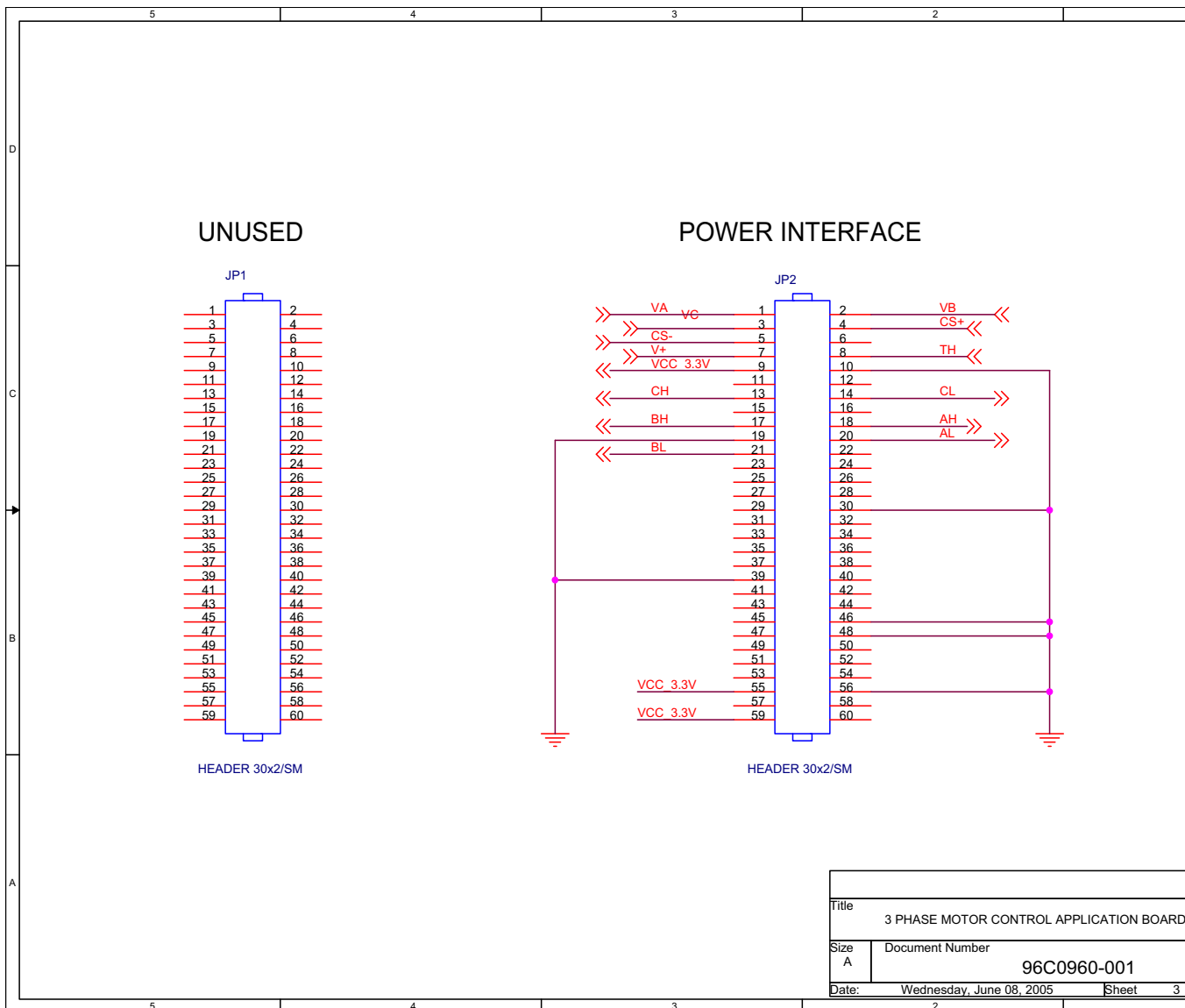
Figure 9. 3-Phase Motor Control Application Board Schematic, #3 of 3
