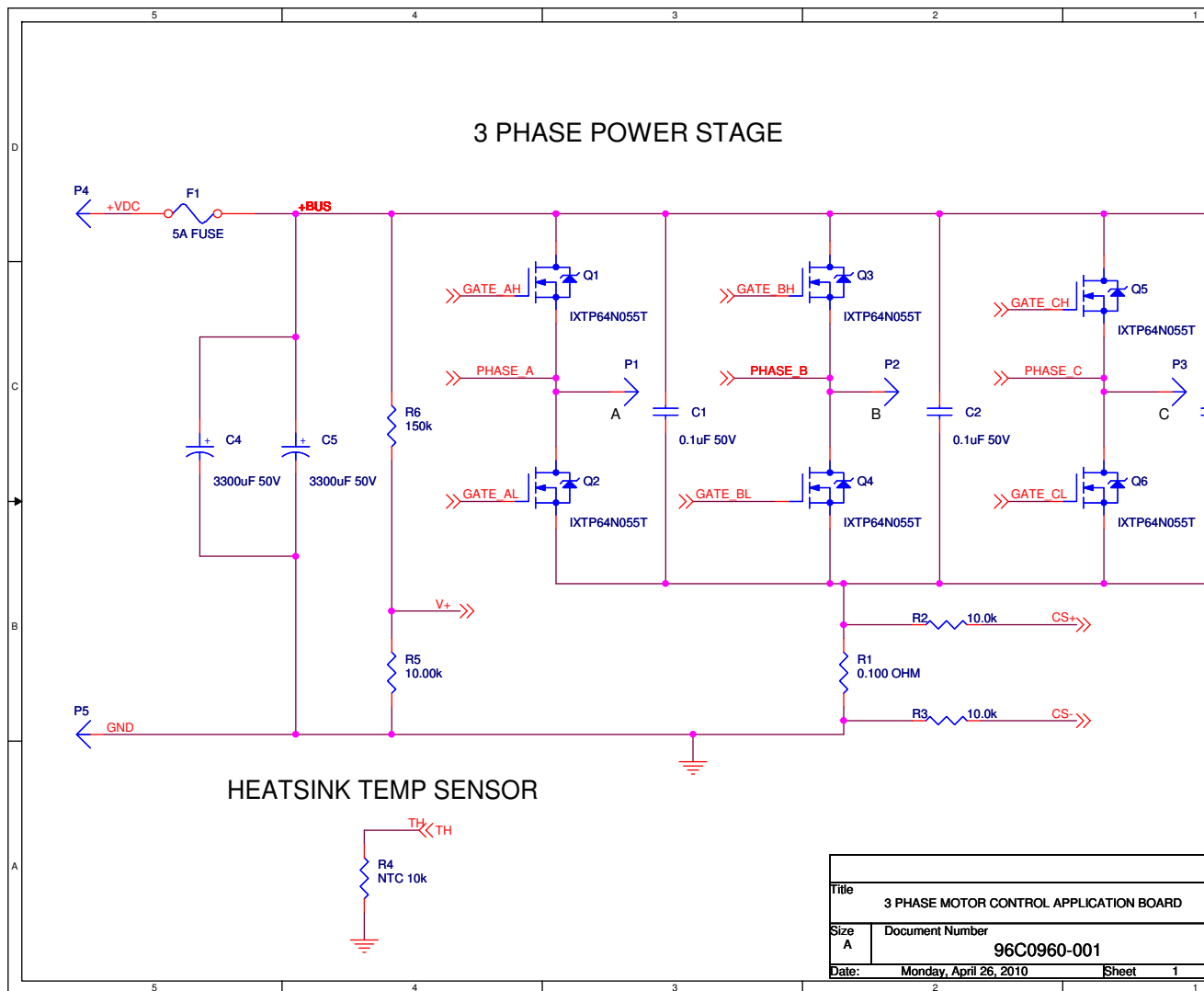
Figure 7. 3-Phase Motor Control Application Board Schematic, #1 of 3
