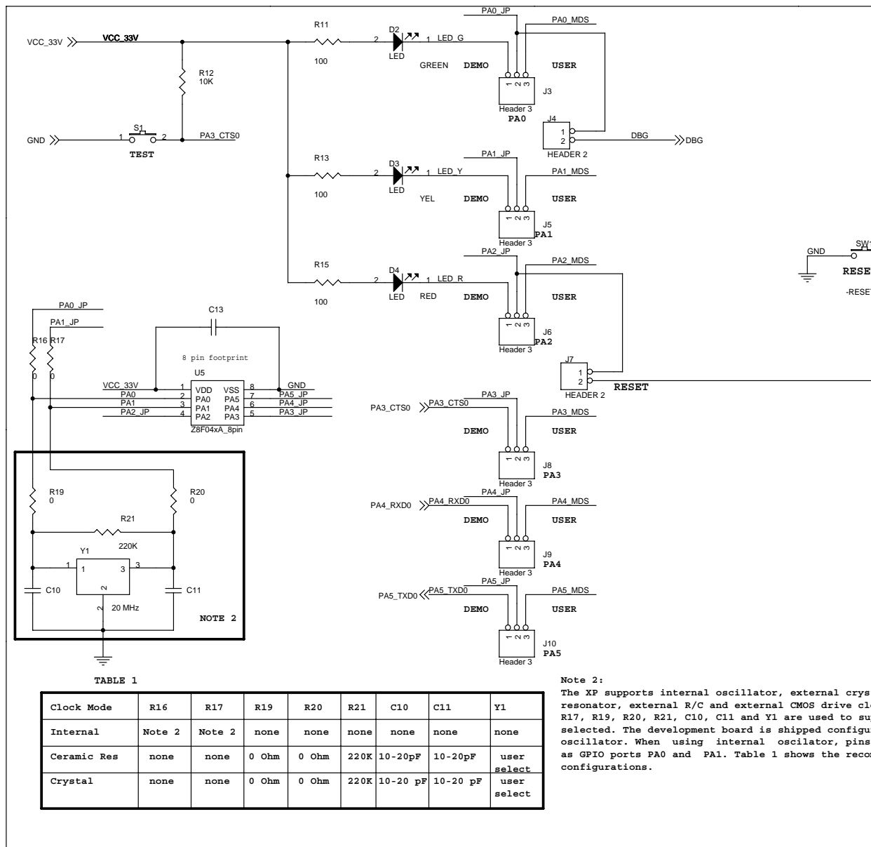
Figure 4. Schematic for Z8 Encore! XP F042A Series 8-Pin MCU D
