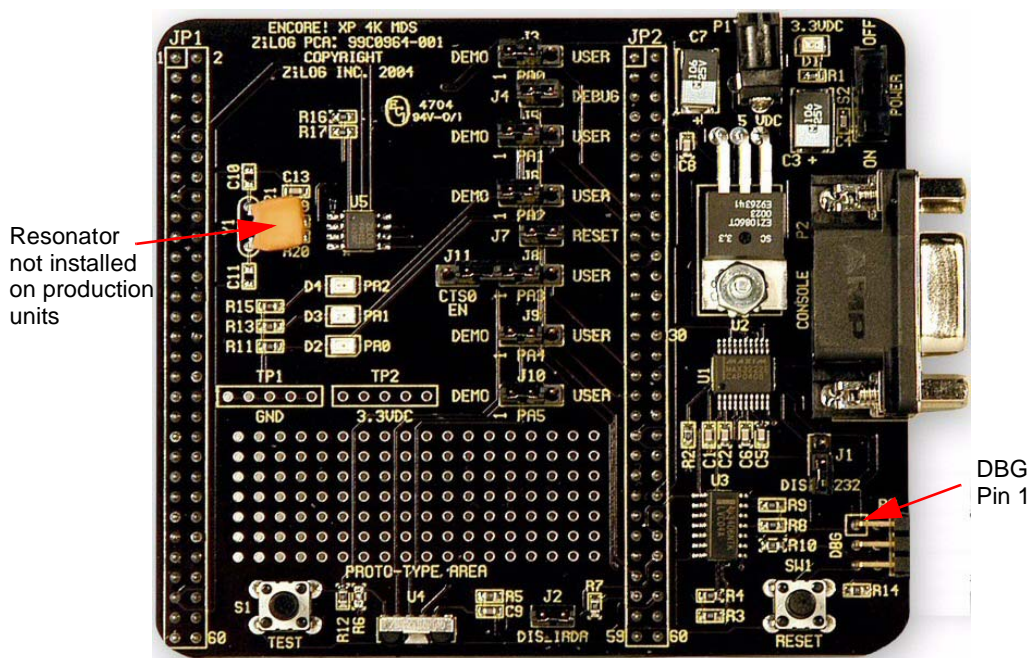
Figure 2. Z8 Encore! XP F042A Series 8-Pin Development Board
