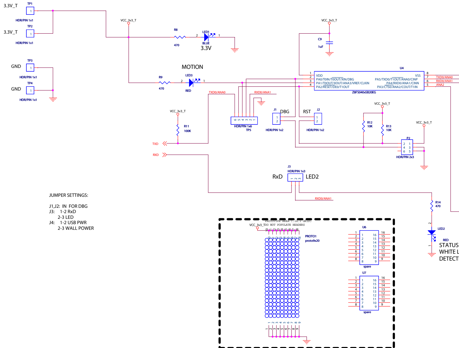
Figure 19. ZMOTION Development Board Schematic Diagram, #2 of 2
