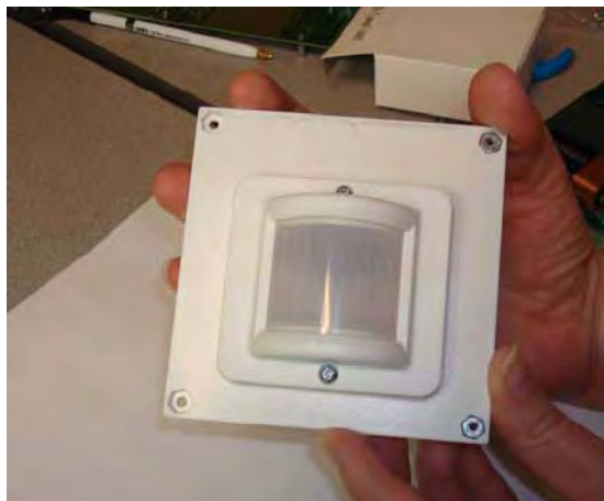
Figure 10. Assembled Flat 0.9" Lens Holder and Flat Lens
