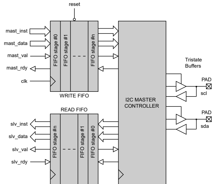
Figure 1: I2C Master serial controller architecture
