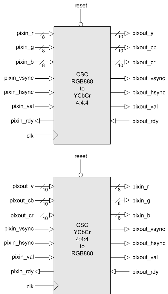
Figure 1: Colour-Space Converter architecture
